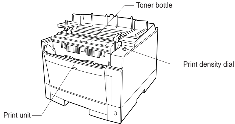
Figure 1-3 Interior view
